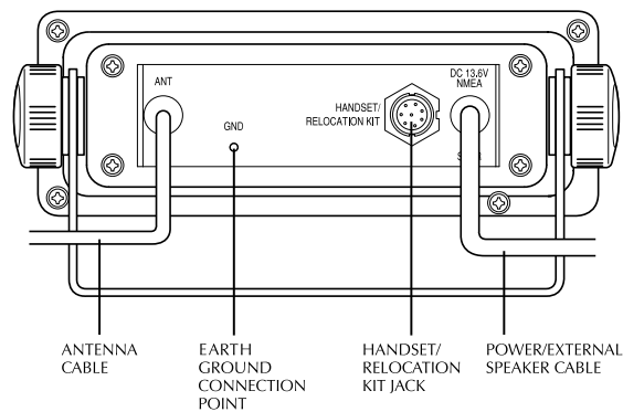
Figure 4-1 Rear Connections
