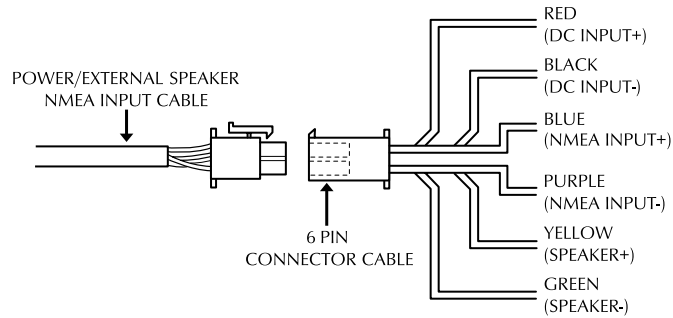
Figure 2-3 Power/External Speaker/NMEA Cable and 6 Pin Connector
