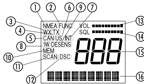
Figure 4-3 LCD Display Layout
