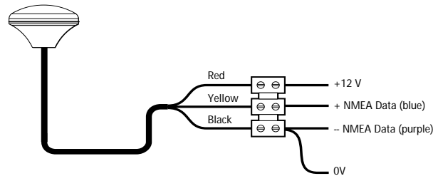
Figure 2-5 GPS Connections
