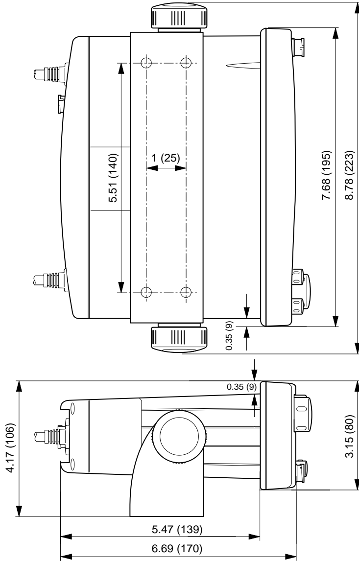
Figure 2-2 Outline and Mounting Dimensions
