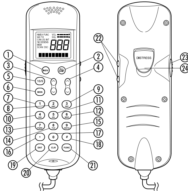
Figure 4-2 Layout of Controls
