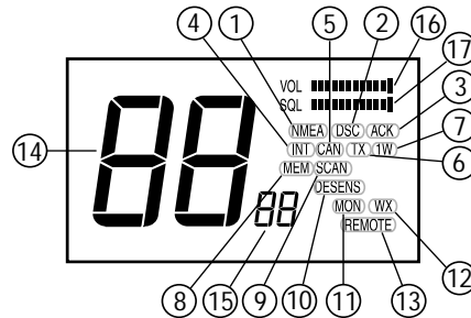
Figure 3-2 LCD Display Layout
