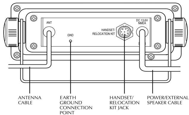
Figure 3-1 Rear Connections
